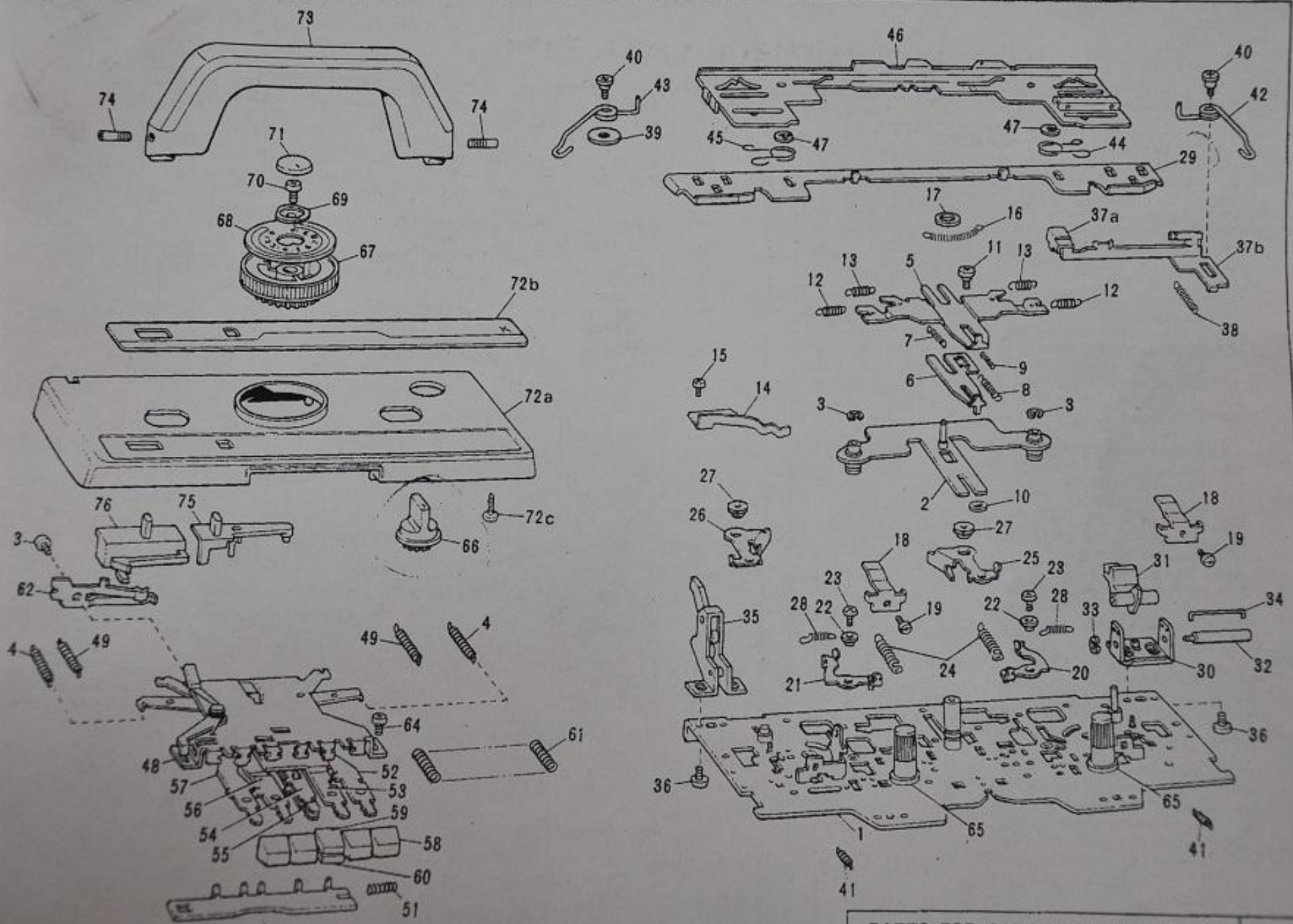
PARTS FOR CARRIAGE UPPER PART Fig. A
