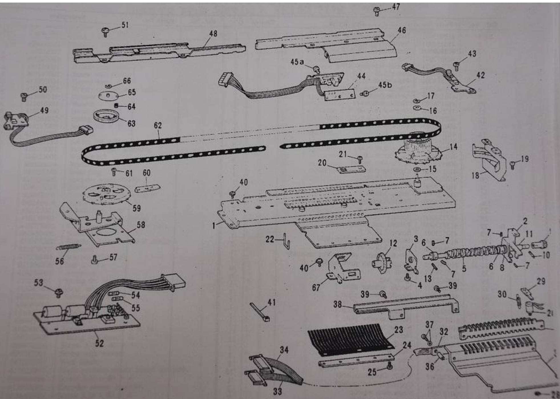
PARTS FOR NEEDLE SELECTOR UNIT Fig
